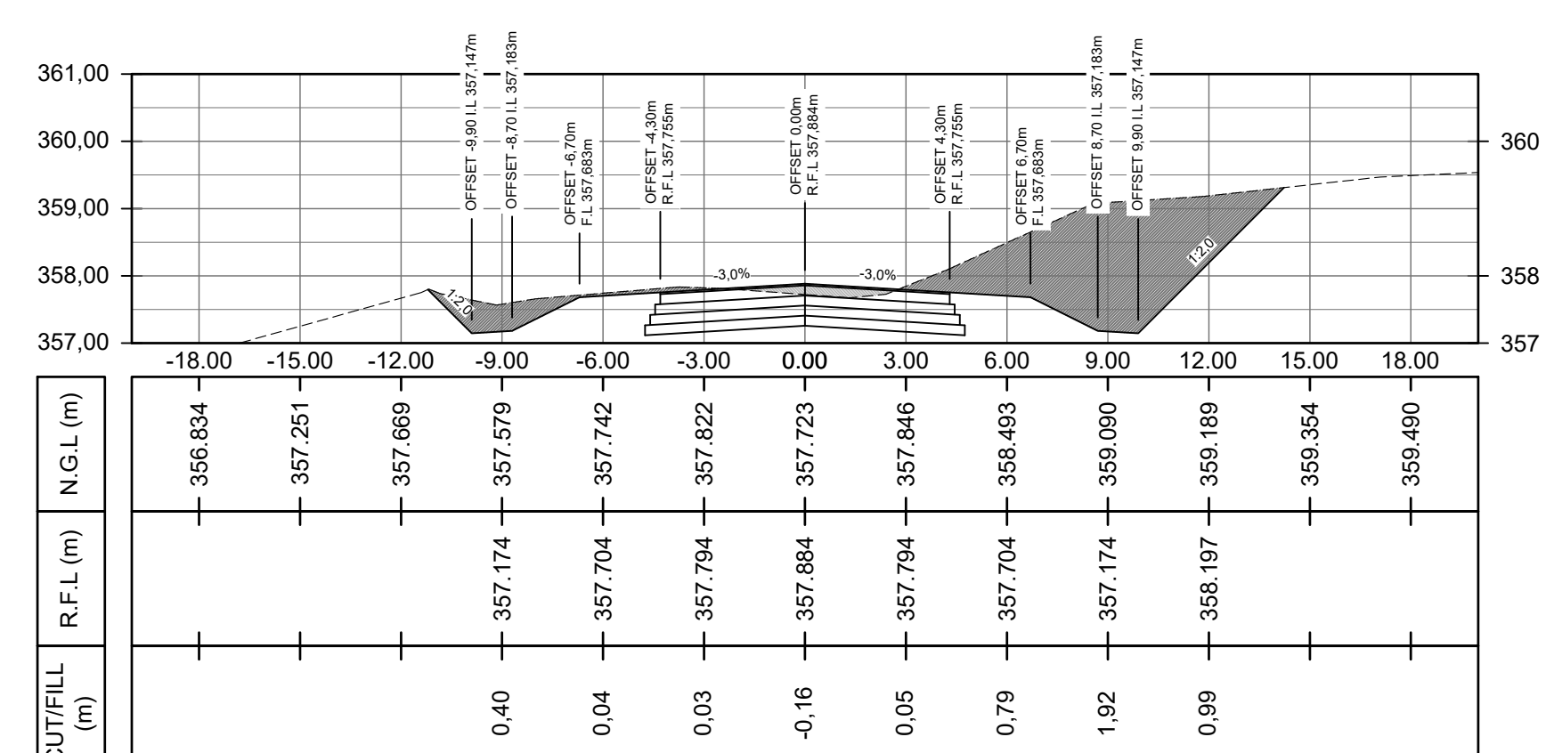
PEG DISTANCE 2900,00m
