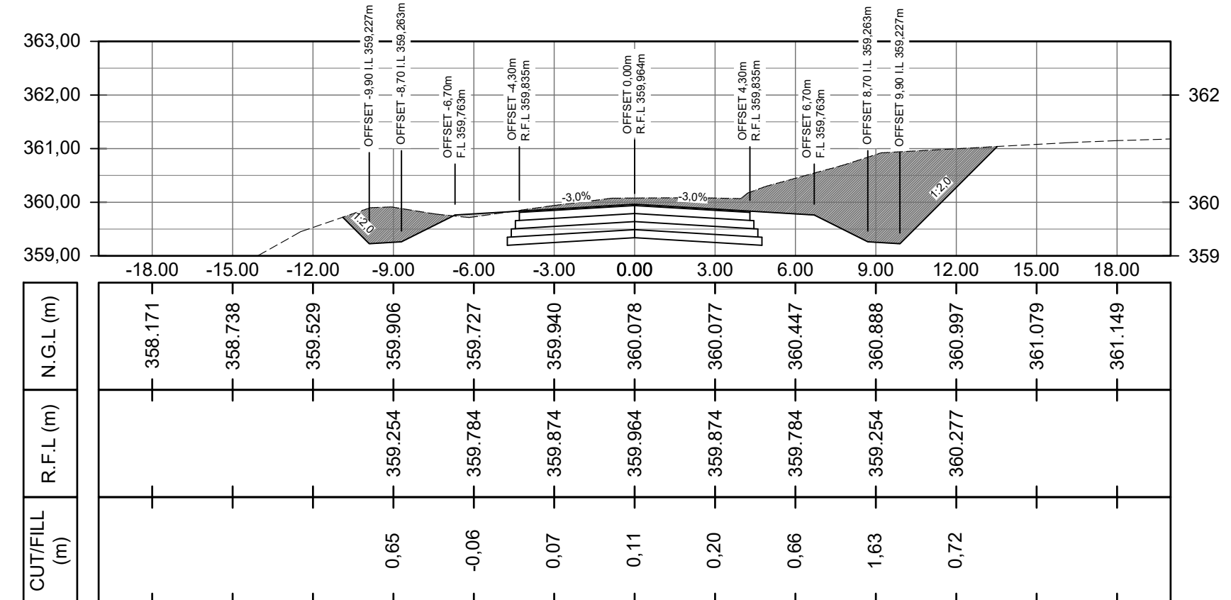
PEG DISTANCE 2840,00m
