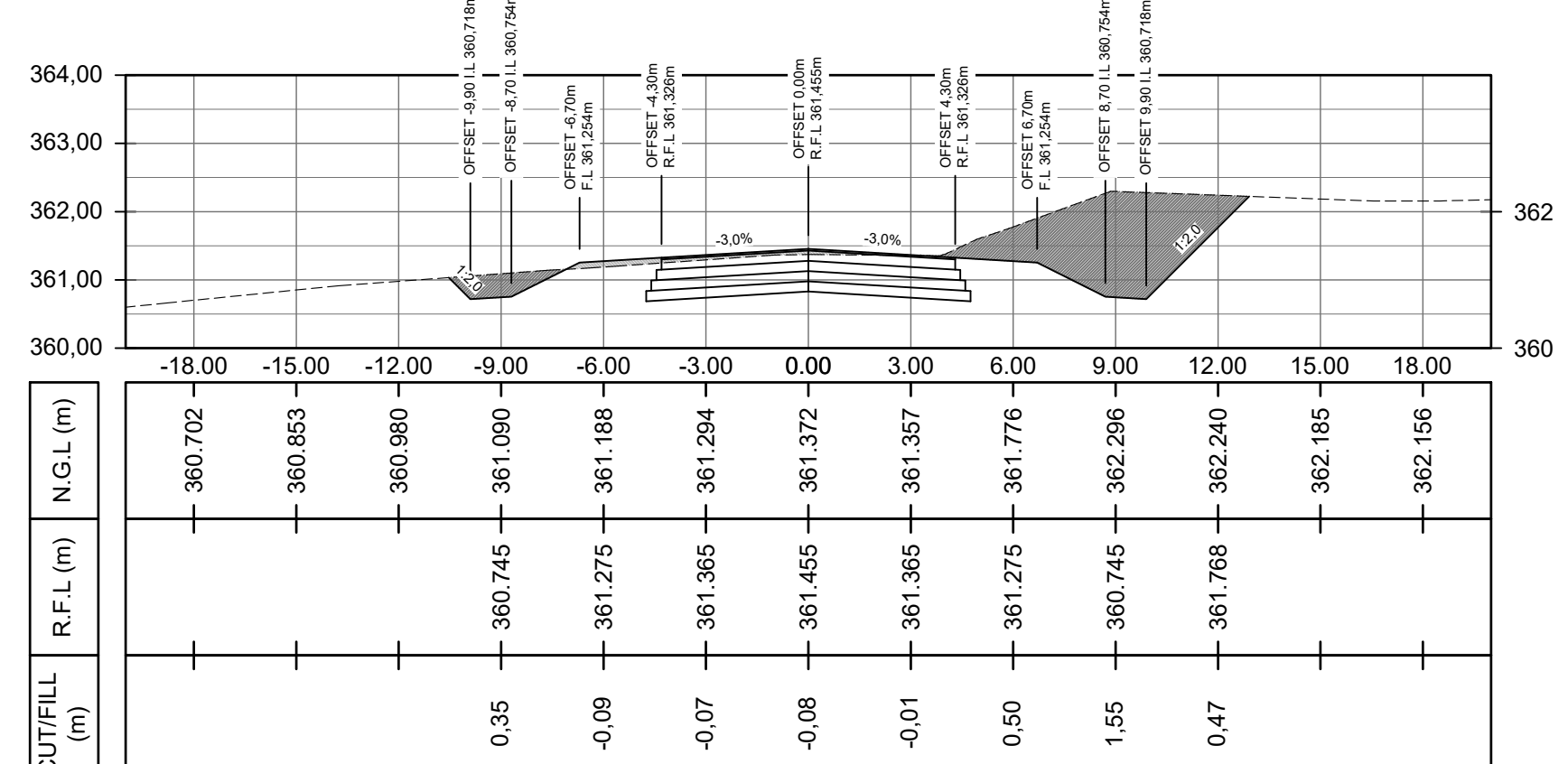
PEG DISTANCE 2800,00m
