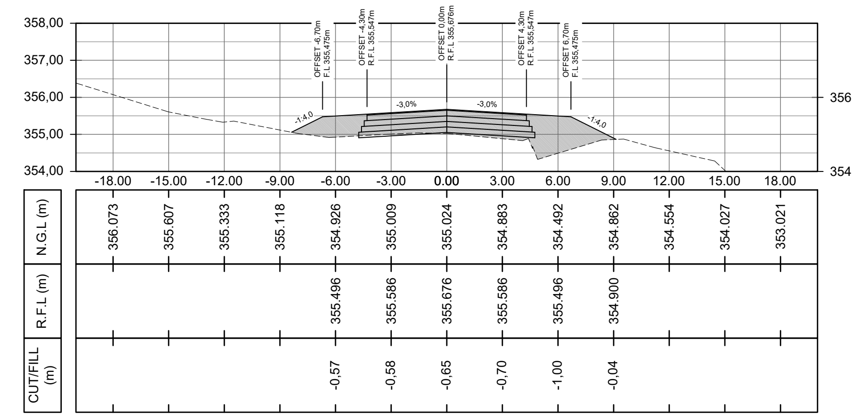
PEG DISTANCE 3060,00m
