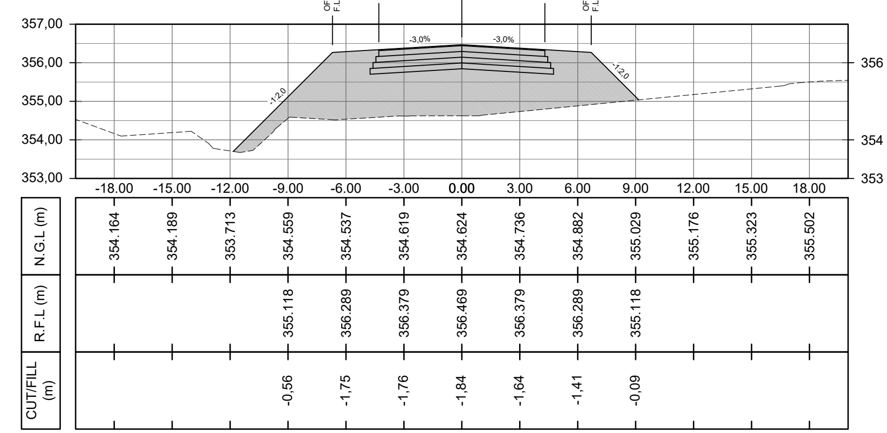
PEG DISTANCE 2960,00m
