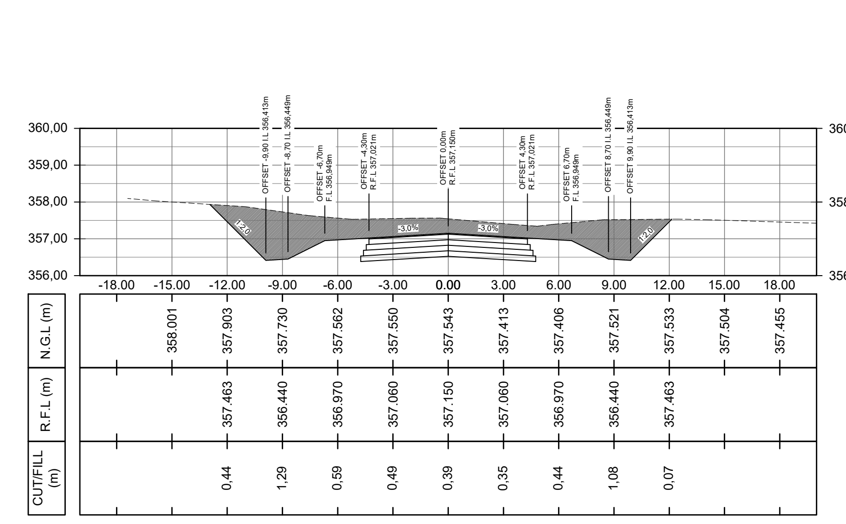
PEG DISTANCE 3180,00m
