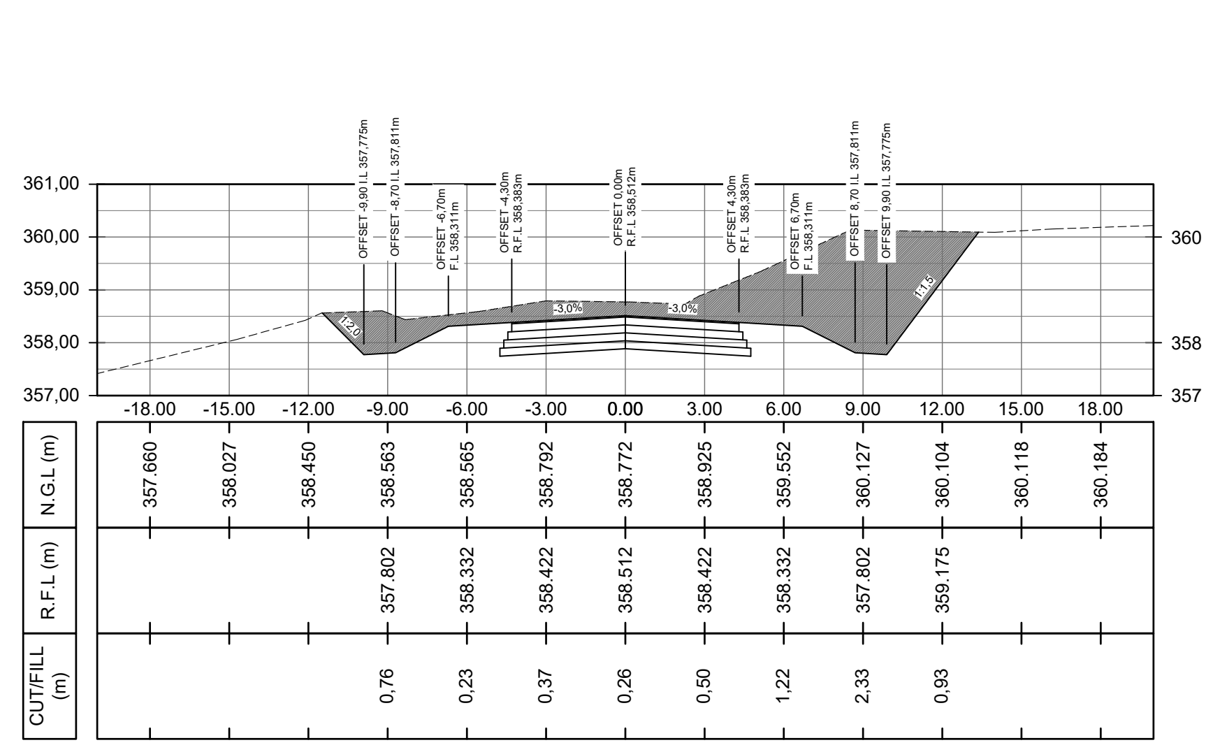
PEG DISTANCE 2880,00m
