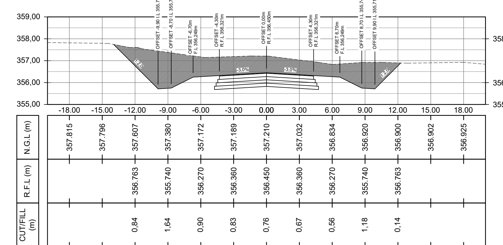
PEG DISTANCE 3140,00m
