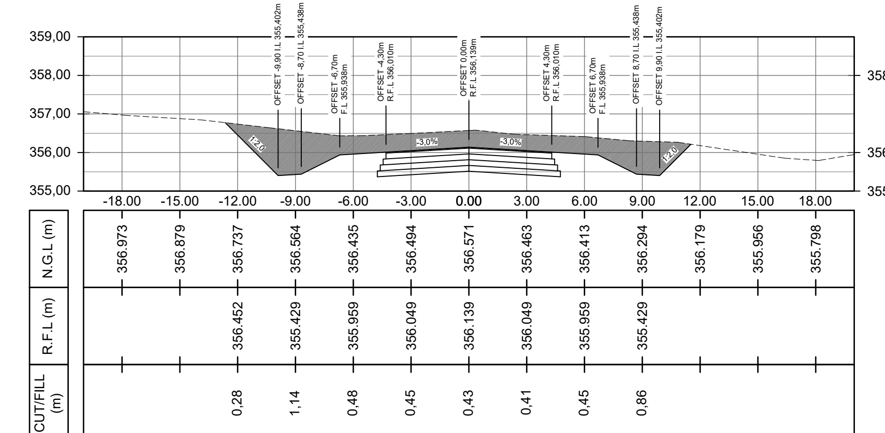
PEG DISTANCE 3120,00m
