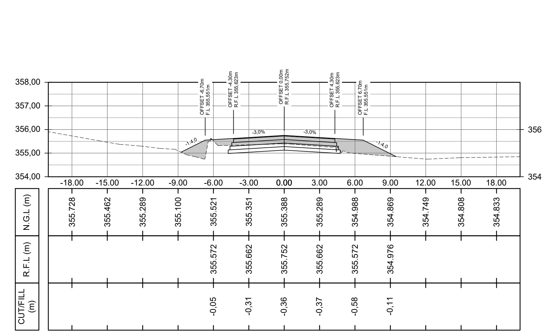
PEG DISTANCE 3080,00m
