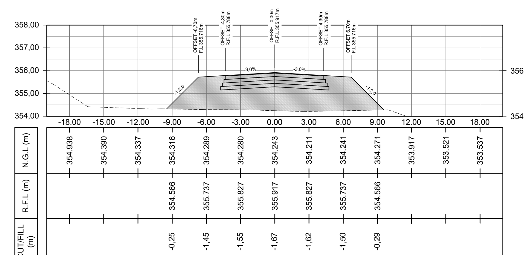
PEG DISTANCE 3020,00m
